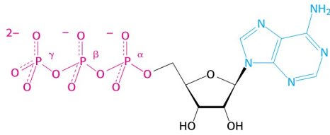
Adenosine triphosphate (ATP)
