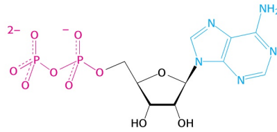
Adenosine diphosphate (ADP)
