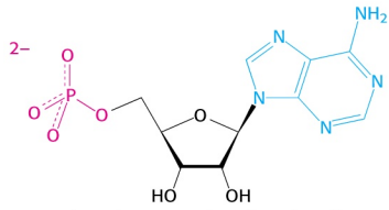
Adenosine monophosphate (AMP)
