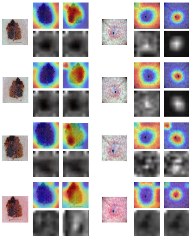
Fig. 7. Examples from the ISIC 2018 data set (top row) and corresponding geometric transformations: horizontal flip (2nd row), 80% central crop (3rd row), and without color normalization (4th row). The first lesion is consistently diagnosed as “Melanocytic Melanoma”, while the second is always diagnosed as “Non-Melanocytic”, but as “BCC” for the first two cases and as “Vascular” in the last two transformations. We also show the spatial attention maps and the most probable activation map for each of the decisions.
