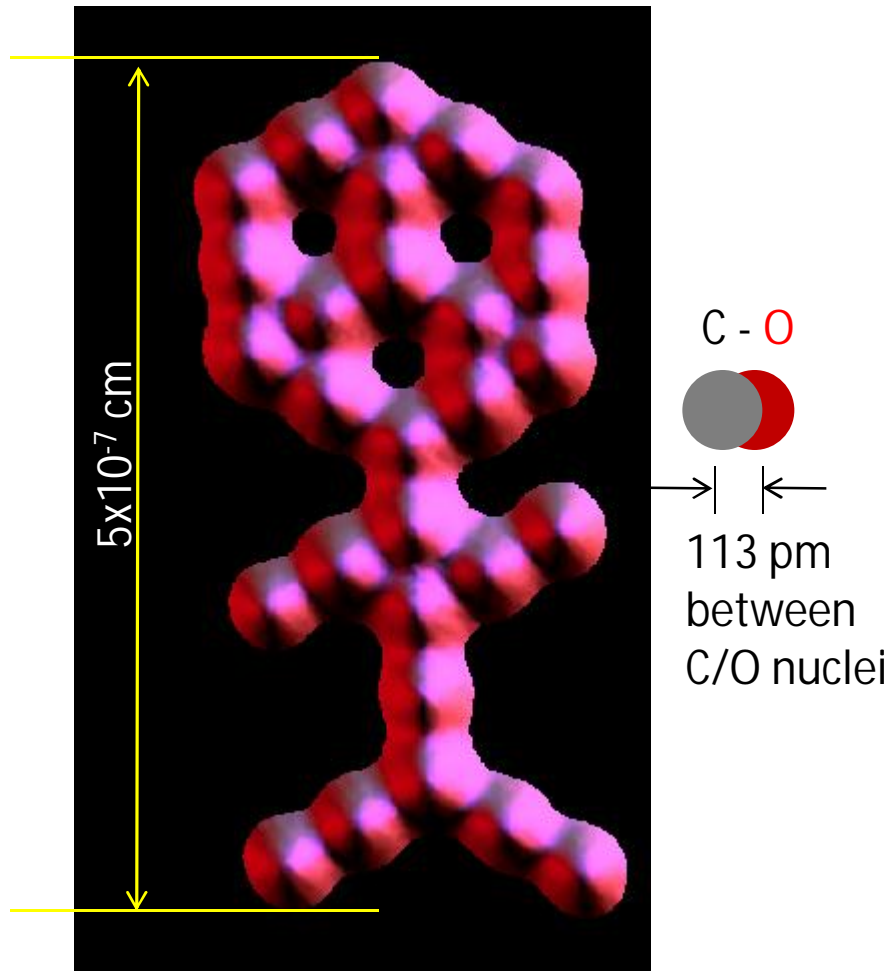
28 CO molecules aligned on a Pt surface using STM to form "Carbon Monoxide Molecule Man"
