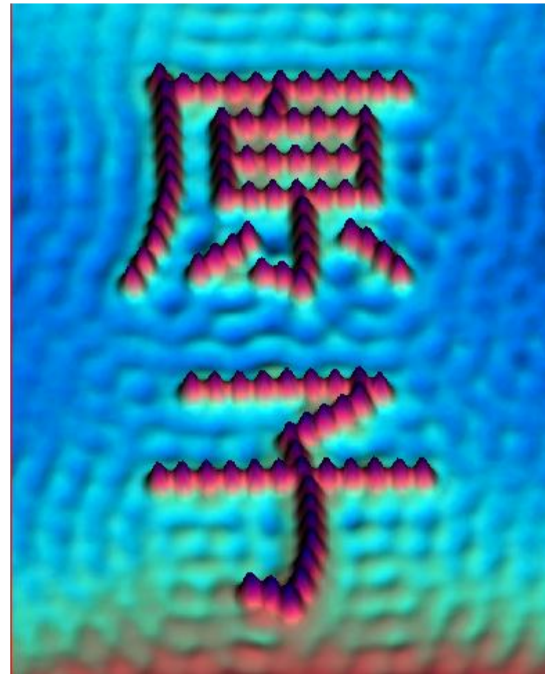
The Kanji characters for "atom" formed with Fe atoms on a Cu surface using STM. Fe atom radius = 126 pm
